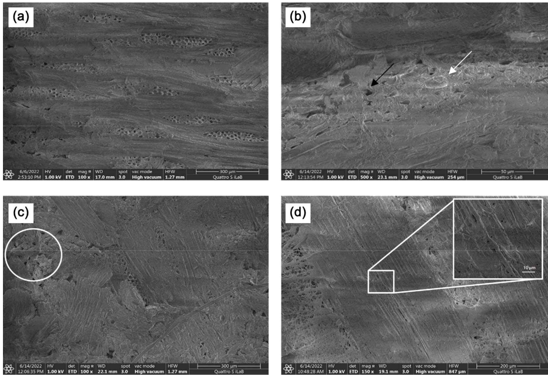
Fig. 4. FE-SEM images of CBPs (bar = 300 \mu\text{m} ). FE-SEM: field-emission scanning electron microscopy, CBPs: chip block pallet.
